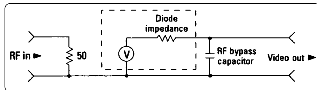
Figure 7. Detector equivalent circuit.
